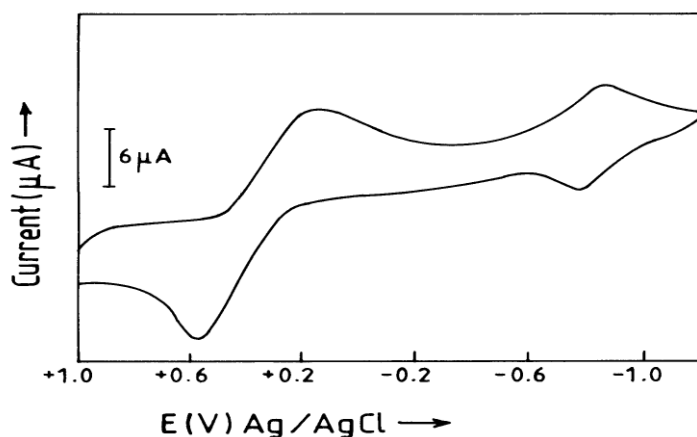
Figure 2: Cyclic voltammogram of copper complex in MeCN
