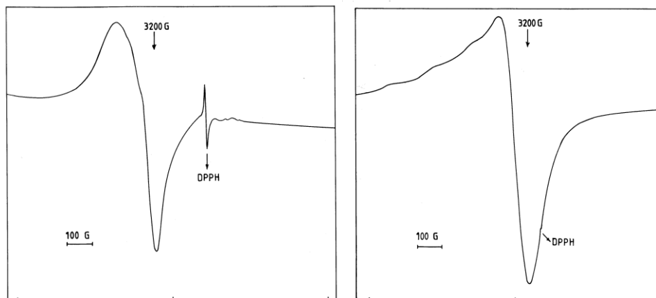
Figure 1: The EPR spectrum of the copper complex in DMSO at 300 K (a) and 77 K (b)
